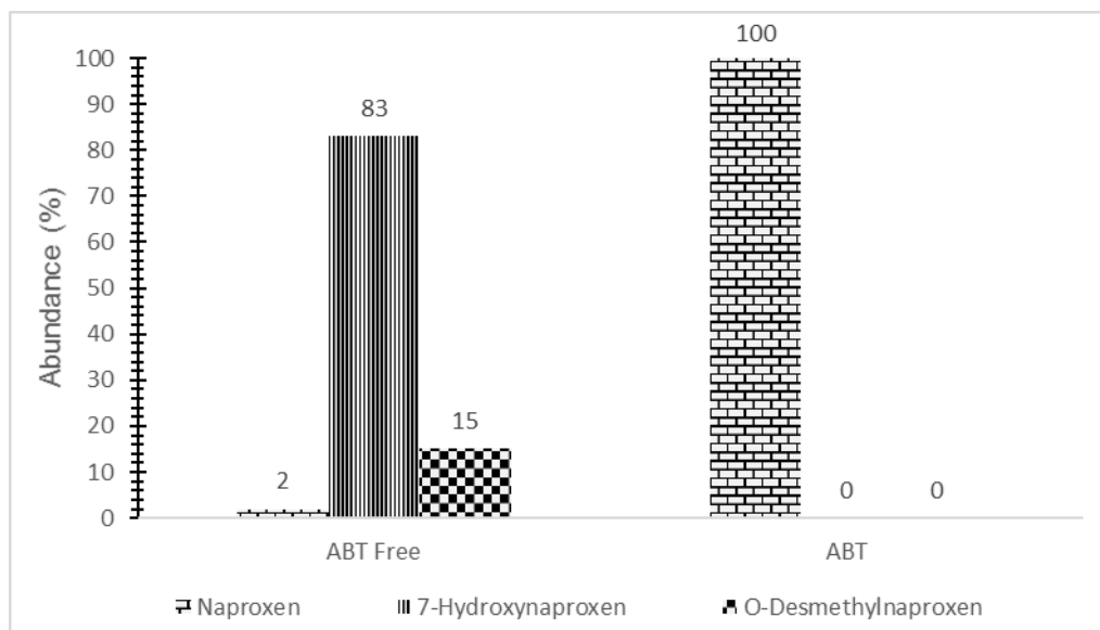
Supplementary Figure. Relative quantities of naproxen and degradation metabolites for 1-Aminobenzotriazole (ABT) containing and ABT free culture mediums in 48h.
