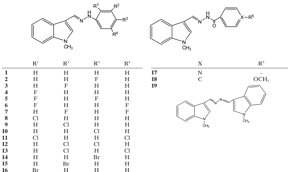
Fig. 1. Chemical structures of compounds 1–19.
