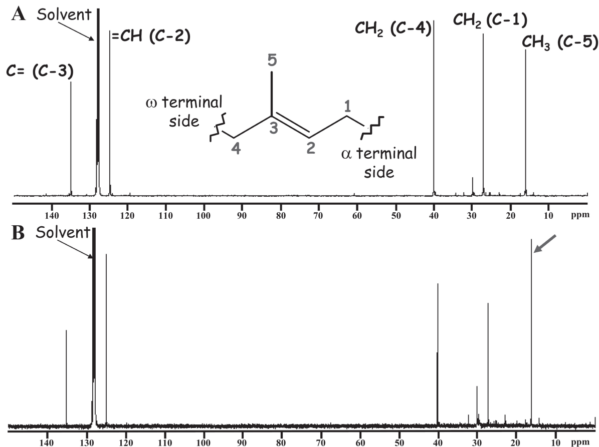
Fig. 5. ^{13}\text{C} NMR spectra of EU -rubber in the feeding experiment with [1-^{13}\text{C}] 1-deoxy-D-xylulose-3,4,5-triacetate (B) and control (A). The signal pointed by an arrow (C-5) increased compared to those of the other positions. [1-^{13}\text{C}] 1-Deoxy-D-xylulose-3,4,5-triacetate was incorporated as an intermediate of the MEP pathway in this feeding experiment (see Fig. 4).
