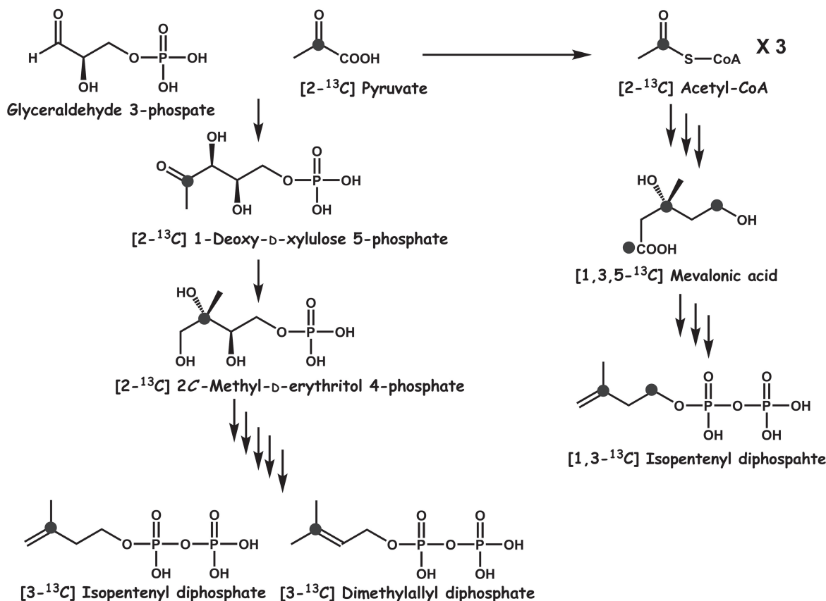
Fig. 7. Predicted labeling patterns of IPP and intermediates of the mevalonate and MEP pathways in the feeding experiment with [2- 13 C] sodium pyruvate.
