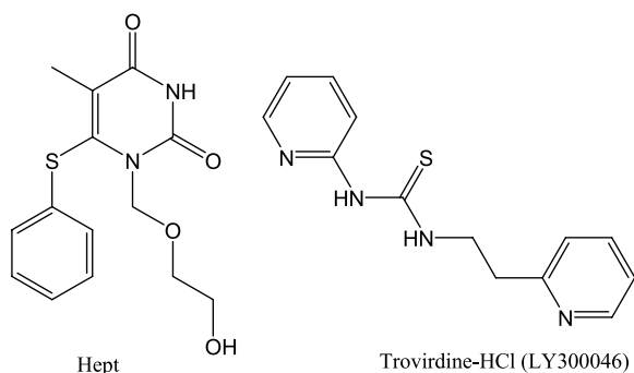
Fig. 1. Chemical structures of Hept and troviridine-HCl (LY300046). Troviridine-hydrochloride (LY300046.HCl) is currently in phase one clinical trials for potential use in the treatment of AIDS. Registries: ChemSpider; InChI-Key HOCFDYZWQYGULA-CUNFQGHECV; PubChem CID 3000870; PubChem ID 197155.
