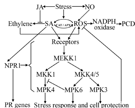
Fig. 2. Hypothetical model showing the role of ROS and SA in the induction of anti-stress gene expression and cell death during abiotic stress. SA can bind and inhibit ROS-removing enzymes, such as CAT and APX, while ROS induces SA directly. SA and H_2O_2 compose a positive feedback. Stress-induced redox regulation is usually accompanied by accumulations of ethylene, NO and JA. Ethylene and NO were found to participate in this SA-ROS self-amplifying loop and the subsequent NADPH oxidase-dependent programmed cell death (PCD). SA promotes ethylene, while JA inhibits SA-induced ethylene biosynthesis and ethylene-mediated PCD. SA signalling is mediated by at least two mechanisms, one requires the NPR1 gene and the second is independent of NPR1 but requires MAPK. SA induces abiotic-stress-protective genes almost through the second mechanism. Transmission of SA signal takes place via at least three MAPK signalling cascades. MPK6 action inhibits MPK4 activation, while MPK3 stimulates SA-signalling. MPK4 is under control of MKK1, and MPK6/3 is under control of MKK4/5. MEKK1 is an upstream activator of MKK1/4/5. Moreover, MAPK and some transcription factors also could be promoted by NPR1 .
