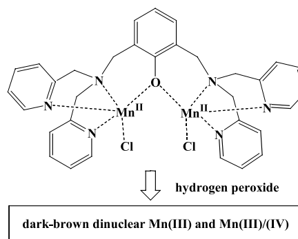
Scheme III.
