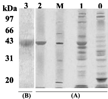
Fig. 3. SDS-PAGE of fusion AFGP in E. coli : (A) Coomassie brilliant blue R-250 staining; (B) periodic acid-Schiff (PAS) staining. Lanes: M, standard marker proteins; 0, lysate of induced culture of E. coli containing empty pET22b(+) vector; 1, cell lysate from E. coli containing pET22(b) with rafgp ; 2 and 3, purified fusion AFGP.
