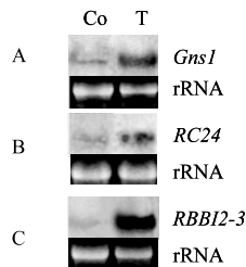
Fig. 5. PR protein genes expression patterns in transgenic rice. 4-Leaf-stage transformants and non-transformants were inoculated with conidiospores of M. grisea . Northern analysis was performed after treated for 72 h; P32-labeled Gns1 , RC24 and RBB12-3 were, respectively, used as probe; 18S ribosomal RNA staining with EB was used as a loading control. Co, control transformant; T, transformant. Expression patterns of (A) Gns1 ; (B) Rc24 ; and (C) RBB12-3 are shown, respectively.
