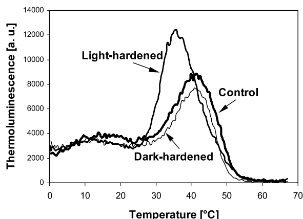
Fig. 1. Effects of cold hardening under different light conditions on the TL curve induced by 30 s FR light in winter wheat plants. TL was recorded at a heating rate of 0.5^{\circ}\text{C s}^{-1} .
