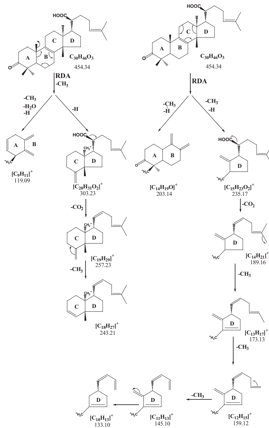
Fig. 2. Proposed EI/MS fragmentation pattern for compound 5.
