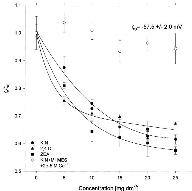
Fig. 1 A. The ratio of zeta potential of polystyrene latex (L 88) after treatment by phytohormone (KIN-kinetin, 2,4-D and ZEA-zearealenone) solutions ( \zeta ) to its value measured in the absence of phytohormones ( \zeta_0 ). Full points correspond to aqueous phytohormone solution, empty points represent the data obtained for kinetin (KIN) in solution containing mannitol, MES and 2 \times 10^{-5} \text{ M Ca}^{2+} . The \zeta / \zeta_0 data represent the average of three separate experiments ( \pm \text{SD} ), counting at least 10 replicates for each experiment.
