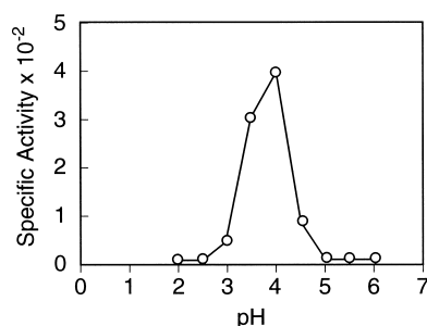
Fig. 4. Determination of the optimum pH of the aspartic proteinase activity on Hb. The enzyme was diluted in 100 mM of following buffers: -sodium citrate (pH 2.5–3.0), sodium acetate (pH 3.5–5.5), Mes (pH 5.0–7.0), -sodium phosphate (pH 6.0–7.5), HEPES (pH 7.5–8.5), and Tris-HCl (pH 7.5–9.5).
