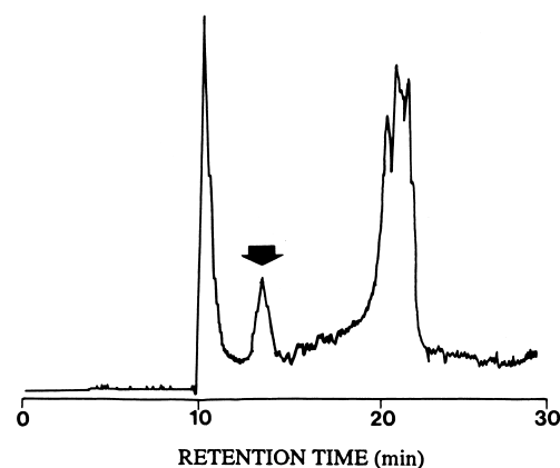
Fig. 3. Gel filtration chromatography analysis of the pepstatin-agarose purified proteinase using a Shinpack Diol-150 HPLC column (50 cm × 7.9 mm I.D.). About 100 µg of protein were analysed and elution performed using 10 mM phosphate buffer (pH 7.3) at a flow-rate of 1 ml·min -1 . Absorbance was measured at 280 nm using AUFS = 4. Protein peak with Hb-hydrolysing activity (retention time of 12.84 min) is indicated. This peak corresponds to a 1.6–1.8% of the total fractioned protein.
