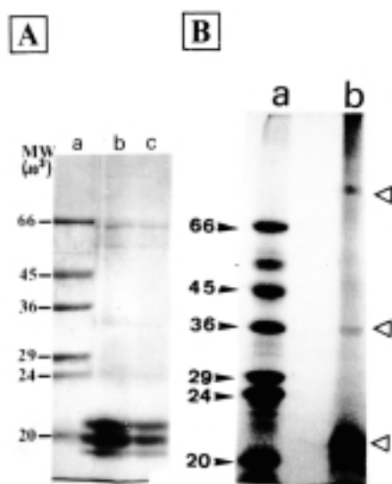
Fig. 2. SDS-PAGE (12.5%) under reducing (A) and non reducing (B) conditions of pooled peak from pepstatin-agarose column followed by staining with Coomassie blue-R 250. Lanes: a, standard molecular weight; b and c, purified proteinase (30 and 10 µg respectively). In the lane Bb about 45 µg of protein was applied.
