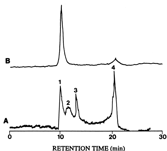
Fig. 5. HPLC of purified 125 kDa protein incubated for 2 h at pH 3.5 (A) and pH 7.0 (B). The chromatographic conditions were the same as in Fig. 3.
