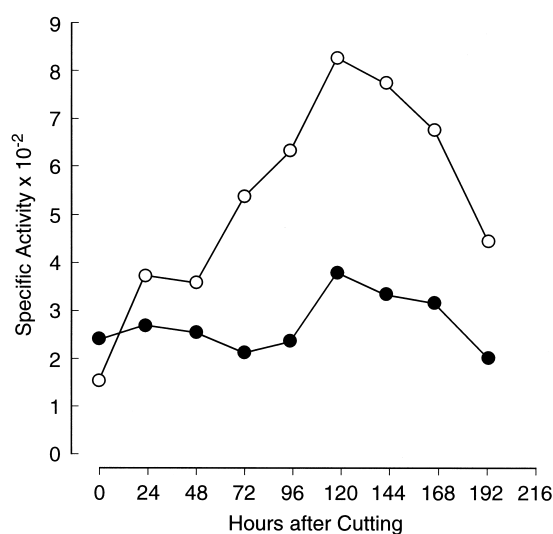
Fig. 1. Profiles of specific activity level of aspartic proteinase during the regeneration of the tail (○—○) and head (●—●) of D. tigrina planaria using haemoglobin as substrate. The enzymatic activity was expressed in OD 280 nm \cdot min -1 \cdot mg protein -1 . The results represent the mean of three experiments.
