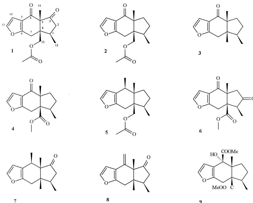
Fig. 1. Pinguisane sesquiterpenes isolated from Porella recurva a and other liverworts b .
