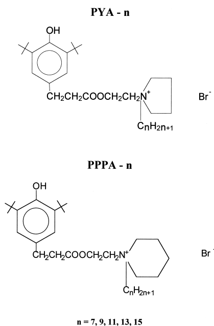
Fig. 1. The compounds studied; pyrrolidinium bromides – PYA- n , piperidinium bromides – PPPA- n .
