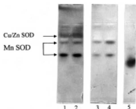
Fig. 4. Electrophoretic migration patterns of SOD of H. polymorpha CBS 4732 cultivated on 1: 8% glucose for 20 h; 2: 1% glucose for 16 h; 3 and 4: the same like 1 and 2 inhibited with 2 mM KCN as described in Materials and Methods; 5: control, Mn SOD from B. stearotheophilus inhibited in the same way.
