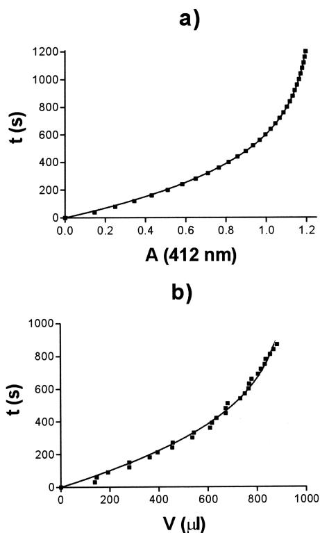
Fig. 2a,b. Hydrolysis of ATCH by BCHE up to high conversion of ATCH. a) Ellman's method: Graphical comparison of the data from the experiment 2 with relation (6), R^2 = 0.9999 . b) pH-stat method: Graphical comparison of the data from the experiment 6 with relation (8), R^2 = 0.9925 .
