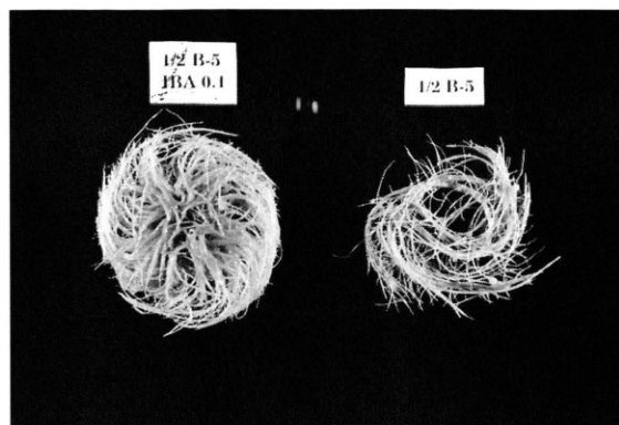
Fig. 2. Hairy roots of Catalpa ovata (HR-1 line) cultured in \frac{1}{2} B5 liquid medium with indole 3-butyric acid (0.1 mg/l IBA) (left) or without IBA (right) for 5 weeks, in the dark (bar = 1 cm).
