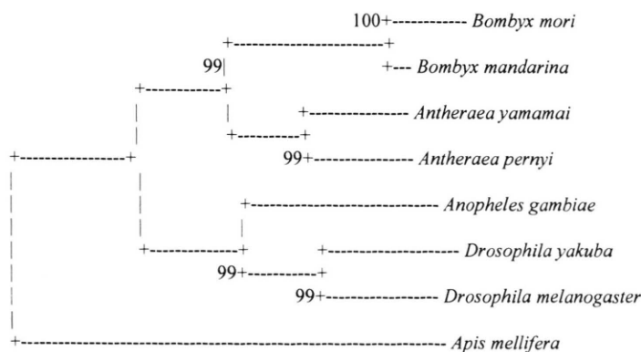
Fig. 3. Dendrogram of the phylogenetic relationships in silkmoths and other insects based on mtDNA cytochrome oxidase I sequence data.
