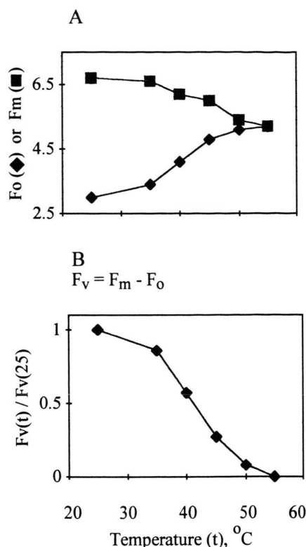
Fig. 1. Effect of temperature on (A) the minimal fluorescence, F_o , and the maximum fluorescence, F_m , and (B) the variable fluorescence, F_v (= F_m - F_o) , in photosystem II particles incubated at temperatures ( t ) between 25 and 55 °C.
