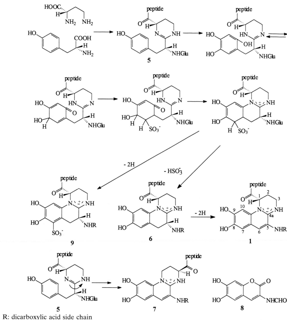
Fig. 2. Proposed biogenetic scheme for the pyoverdine chromophore.
