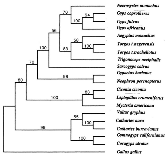
Fig. 2A. Reconstruction of phylogenetic relationships between vultures and storks by maximum parsimony (MP), UPGMA and neighbour-joining (NJ) based on 1026 bp of the cytochrome b gene. Gallus gallus was used as an outgroup.
