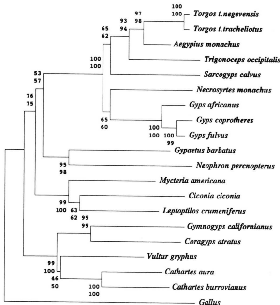
Fig. 2C. NJ, Percent bootstrap frequencies (500 replicates) are indicated above each furcation; upper values are based on Kimura two-parameter, lower value on p-distance method. Illustration as a phylogram; branch lengths are proportional to genetic distances. The distance algorithm Tamura-Nei produced a tree of almost identical topology. Abbreviations as in Fig. 1.
