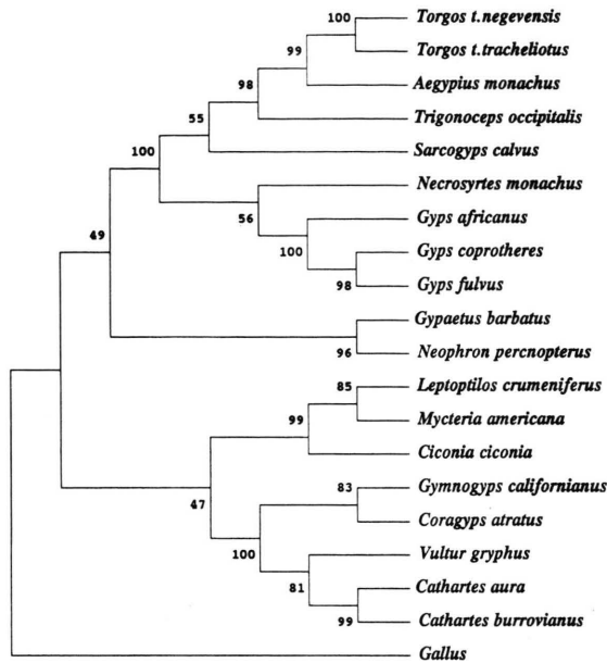
Fig. 2B. UPGMA, The phenetic relationships are shown as a cladogram; bootstrap values (500 replicates) are given at each nodes. (Note, UPGMA trees do not represent phylogenetic trees).
