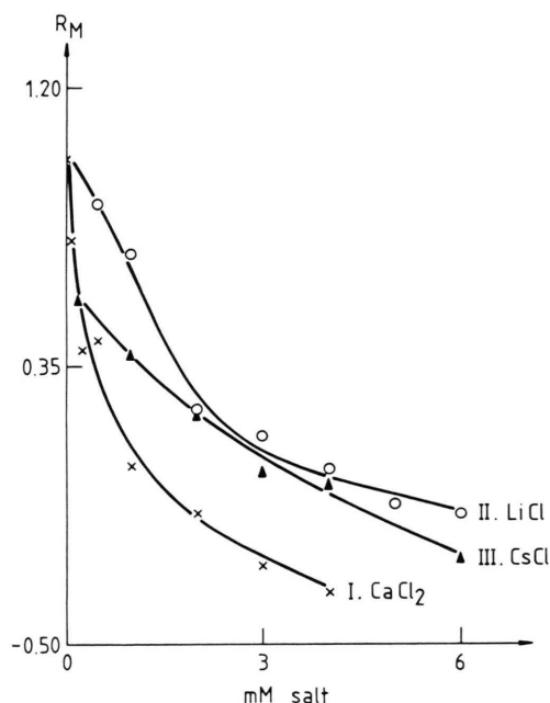
Fig. 5. Effect of salt concentration on the R_M value of 10 \mu g paraquat on cellulose + gliadin layers. I. \text{CaCl}_2 , II. \text{LiCl} , III. \text{CsCl} .
