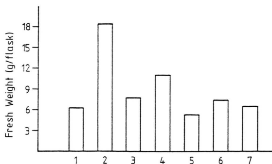
Fig. 4. Growth of an axenic culture of Ricciocarpos natans on different mineral media. Fresh weight (g/flask) after a 35 days' culture period. 1 = Bennecke's medium; 2 = Gamborg B5 medium; 3 = Knop's medium; 4 = Knudsen's medium; 5 = Lorenzen's medium; 6 = MSK-2 medium; 7 = White's medium.
