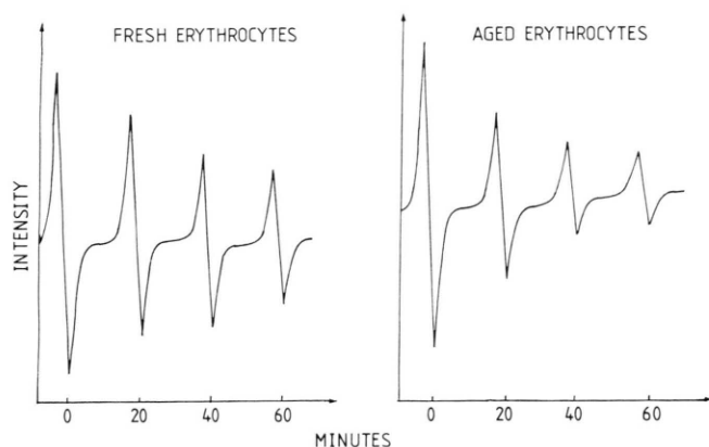
Fig. 5. ESR spectra as function of time expressed as arbitrary units from fresh erythrocytes (left panel) and aged erythrocytes (right panel) treated with MAL-6. [\text{MAL-6}] = 2 \times 10^{-4} \text{ mol} \times \text{dm}^{-3} .
