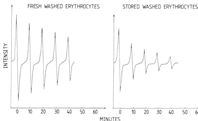
Fig. 4. ESR spectra as function of time expressed as arbitrary units from washed erythrocytes treated with MAL-6. Left panel, fresh washed erythrocytes; right panel stored washed erythrocytes [\text{MAL-6}] = 2 \times 10^{-4} \text{ mol} \times \text{dm}^{-3} .
