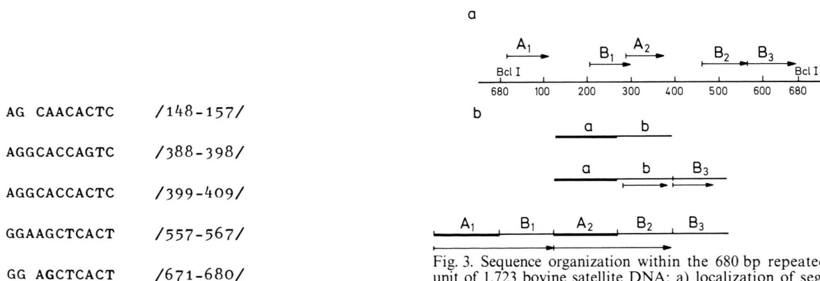
Fig. 2. Regions of significant homology scattered on the 680 bp unit and their positions.
