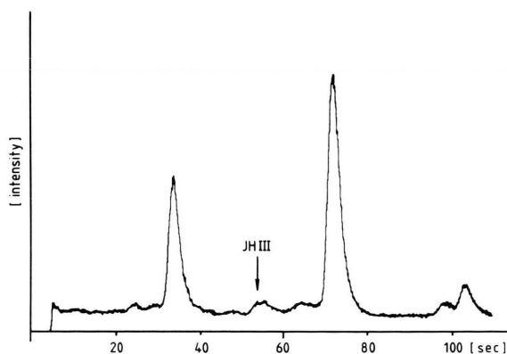
Fig. 4. MIS plot for the fragment m/e 376 formed from the 10-nonafluorohexyldimethylsilyl-11-methoxy-JH-III derivative after separation by GC (245° const., capillary column Durabond-1, 0.25 mm i.d. , 30 m) – MS in EI mode (0.05 pmol JH-III). For more technical details comp. (12). Retention time of the resp. JH-III ethyl ester (1.2 pmol) is at 73 s.
