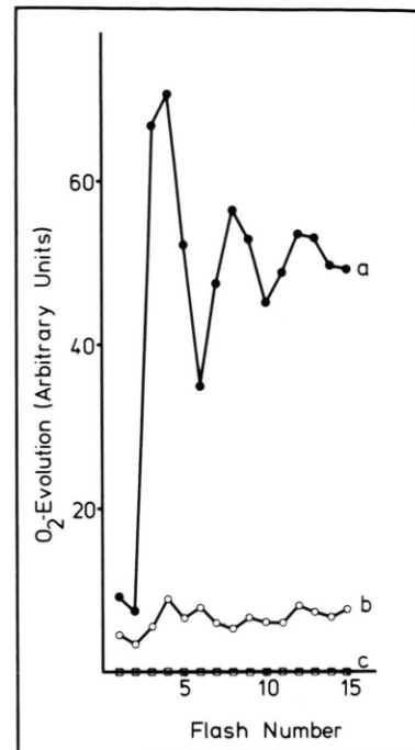
Fig. 3. Effect of 10 \mu\text{M} CCCP (○) and 20 \mu\text{M} CCCP (□) on the flash sequence of Oscillatoria chalybea . (●) control sequence. Dark adaptation 15 min.
