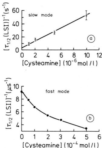
Fig. 7. Influence of cysteamine on the rate of LSI decrease in \text{N}_2\text{O} -saturated aqueous solution of poly A (0.3 g/l, \bar{M}_w = 6.8 \times 10^5 ) at pH 7.8 and 23^\circ\text{C} . Reciprocal half-life of the slow mode (a) and of the fast mode (b) of the LSI decrease vs. the concentration of cysteamine hydrochloride. [phosphate buffer] = 5 \times 10^{-3} mol/l; [\text{NaClO}_4] = 1 \times 10^{-2} mol/l; absorbed dose per pulse: 10.5 Gy (a) and 37 Gy (b).
