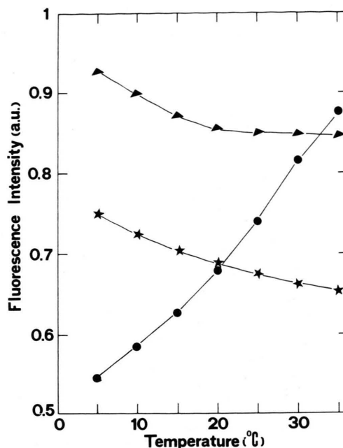
Fig. 3. The effect of temperature on the HP fluorescence emission yield in absolute methanol ( \blacktriangle ), 90% methanol ( \star ), and 0.05 M phosphate buffer at pH 7.4 ( \bullet ). The spectra were excited at 440 nm, using 7 nm and 8 nm spectral bandwidths for the excitation and emission light, respectively. Each sample was kept at the desired temperature for at least 10 min prior to measurement in order to ensure the attainment of thermal equilibrium.
