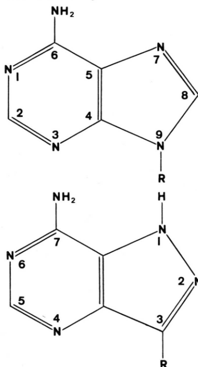
Scheme 1. Showing structural analogy between adenosine (above, R = ribose) and formycin (R = ribose). With R = alkyl, we have the corresponding 9-alkyladenine and 3-alkylpyrazolo(4,3-d)pyrimidine.
