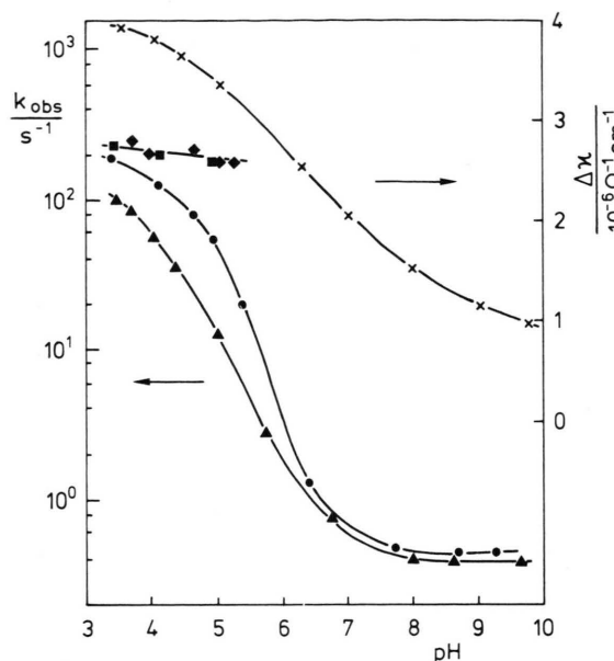
Fig. 6. \text{pH} -Dependence of the conductivity-increase \Delta\kappa (right ordinate) and of the logarithm of its rate constant (left ordinate) measured after 1 \mu\text{s} electron pulses of 10 \text{ J kg}^{-1} dose in aqueous \text{N}_2\text{O} -saturated solution of poly U at 18^\circ\text{C} . \times \times refers to the right ordinate and was measured with the potassium salt of polyribouridylic acid (= poly U) at 60 \text{ mg l}^{-1} . The filled symbols refer to the left ordinate: \blacktriangle \blacktriangle = 60 \text{ mg l}^{-1} poly U; \bullet \bullet = 12 \text{ mg l}^{-1} poly U; \blacksquare \blacksquare = 6 \text{ mg l}^{-1} potassium ion free polyribouridylic acid with \text{HClO}_4 added; \blacklozenge \blacklozenge = stock solution of 120 \text{ mg l}^{-1} potassium ion free polyribouridylic acid diluted with distilled water.
