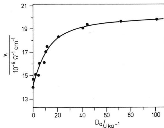
Fig. 1. Conductivity \kappa as a function of dose measured one hour after ^{60}\text{Co} - \gamma -irradiation (dose rate 22 J kg -1 min -1 ). Aqueous N 2 O-saturated solutions of poly U (60 mg l -1 ) at 18 °C and pH = 6.5.
