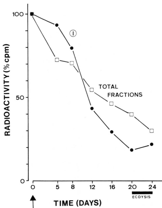
Fig. 2. Time-course of disappearance of [ ^{14}\text{C} ]β-carotene I during the fifth juvenile instar of C. morosus : radioactivity associated with the carotene zone expressed as a percentage of the total activity of all carotenoids (filled symbols). Recovery of radioactivity in the total carotenoid fractions expressed as a percentage of the radioactivity of the total extract (open symbols). Labelled β-carotene was fed (arrow) two days after the fourth ecdysis. Mean-values of duplicate determinations from a single experiment.
