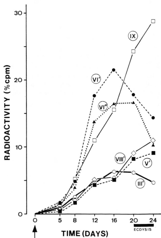
Fig. 3. Time-course of label incorporation from [ ^{14}\text{C} ]β-carotene into the carotenoids III , V , VI , VIII , and IX ( cf. Table I) in C. morosus during the fifth juvenile instar. Labelled β-carotene was fed (arrow) two days after the fourth ecdysis. Radioactivity in a single carotenoid is expressed as a percentage of the total activity of all carotenoids of an extract. Mean-values of duplicate determinations from a single experiment. Primed numbers refer to esters of the corresponding carotenoids.
