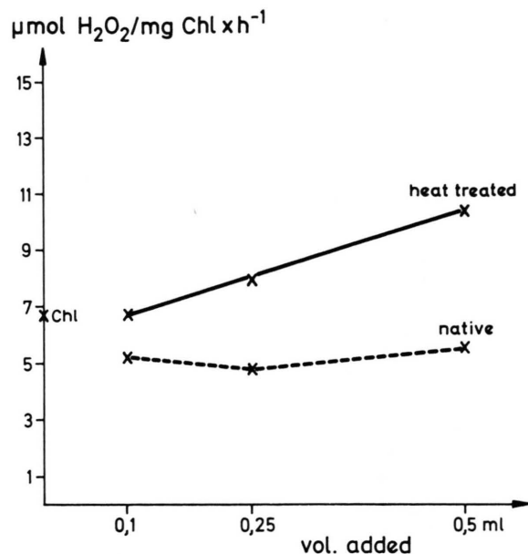
Fig. 8. Stimulation by heat-treated ferredoxin-NADP reductase of H_2O_2 production by illuminated chloroplast lamellae. 2 ml ferredoxin-NADP reductase with ca 6.5 mg protein were heat-treated (5 min at 80 °C) and centrifuged (15 min at 5000 \times g ). 1 ml SN corresponded to 3.7 mg protein with a diaphorase activity ( cf. ref. [39]) of units \times mg protein -1 .
