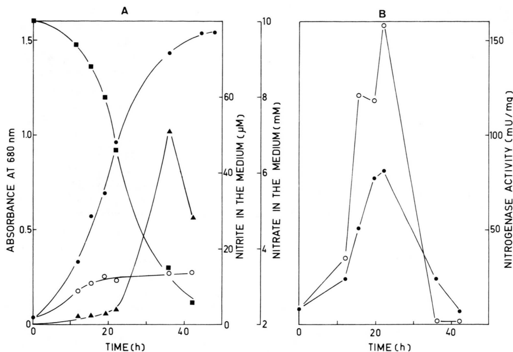
Fig. 2. A) Growth representation and time courses of nitrate uptake and nitrite excretion by R. capsulata E 1 F 1 cells growing anaerobically in the light with or without nitrate in media not sparged with argon. ■—■, nitrate in the medium; ▲—▲, nitrite in the medium; ●—●, absorbance of cultures with nitrate; ○—○, absorbance of cultures without nitrate. B) Time course of nitrogenase activity in whole cells of R. capsulata E 1 F 1 cells growing anaerobically in the light in media not sparged with argon. ●—●, cultures with nitrate; ○—○, cultures without nitrate.
