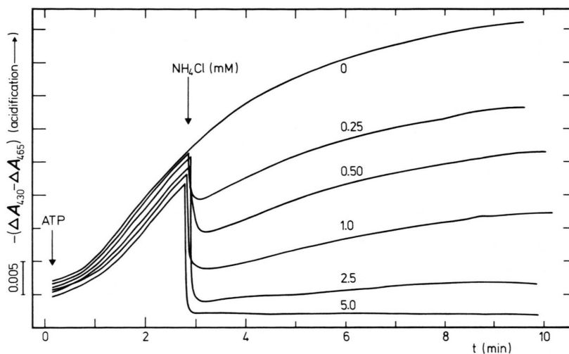
Fig. 6. Reversal of the ATP-induced drop in pH in vesicles through NH 4 Cl ("uncoupling effect").
