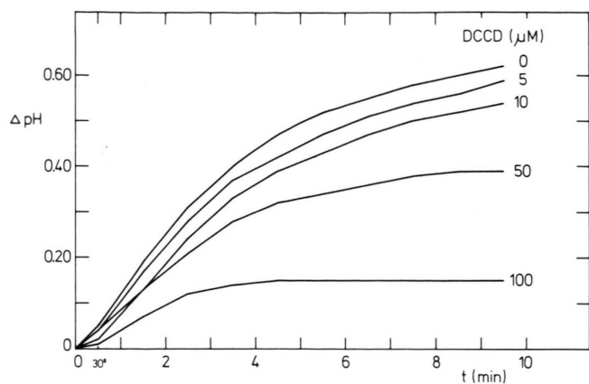
Fig. 3. Inhibition of ATP-dependent acidification in microsomal vesicles by DCCD. Conditions as described for Fig. 1.
