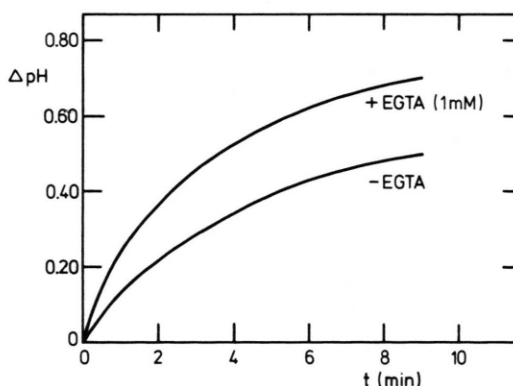
Fig. 2. Promotion of ATP-dependent acidification in microsomal vesicles through EGTA. Conditions as described for Fig. 1 except that the homogenization medium (II) is without and medium IV with or without EGTA (1 mM).
