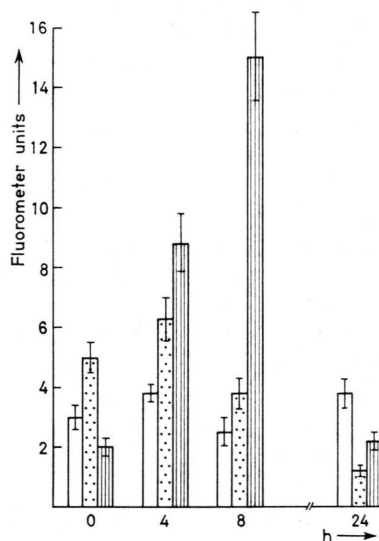
Fig. 3. Effect on pteridine and riboflavin concentration of amphetamine. □: tetrahydrobiopterin; [·]: isoxanthopterin; ▨: riboflavin. Values refer to the mean \pm standard error of the mean of three determinations.
