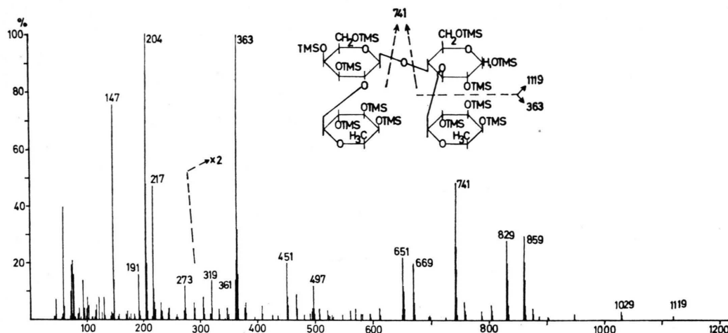
Abb. 5. 20 eV Massenspektrum der Pertrimethylsilyl-O- \alpha -L-fucopyranosyl-(1 \rightarrow 2)-O- \beta -D-galaktopyranosyl-(1 \rightarrow 4)-[O- \alpha -L-fucopyranosyl-(1 \rightarrow 3)]-D-glucose, TMS-3,2'-difucosido-lactose.
