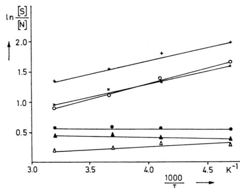
Fig. 6. Van't Hoff plot of the mole fractions of S and N states of the ribose in: 8-BrA ( \times ); 8-BrG ( + ); F ( \circ ); A ( \triangle ); I ( \bullet ); X ( \blacktriangle ).
