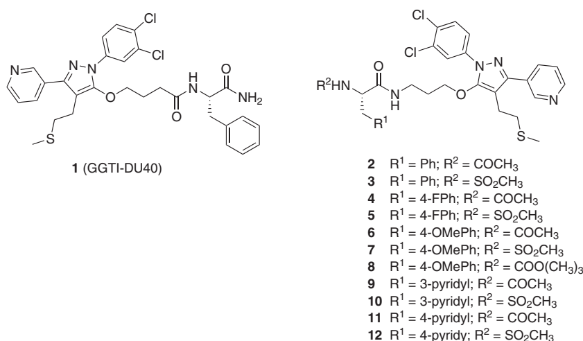
Fig. 1: Structural analogues of GGTI-DU40 ( 1 ).
