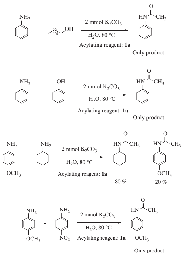
Scheme 2: Chemoselective acylation of amine and alcohol or phenol in the presence of K_2CO_3 in water at 80 °C.
