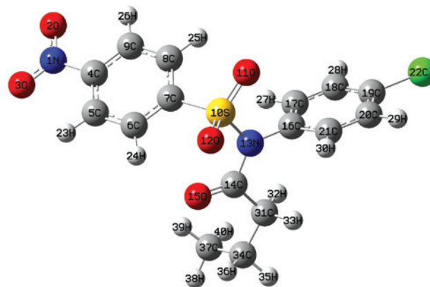
Fig. 1: The optimized structure of N -butyl- N -(4-chlorophenyl)-4-nitrobenzenesulfonamide ( 1b ).
