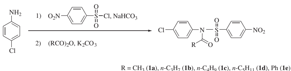
Scheme 1: Synthesis of N -acyl- N -(4-chlorophenyl)-4-nitrobenzenesulfonamides ( 1a–e ).
