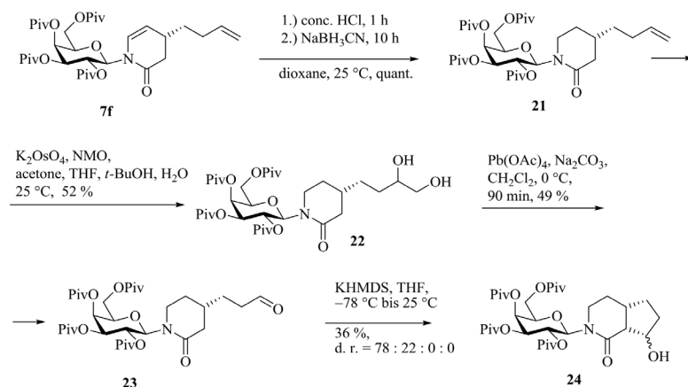
Scheme 11. 3,4-Annulated piperidinones.
