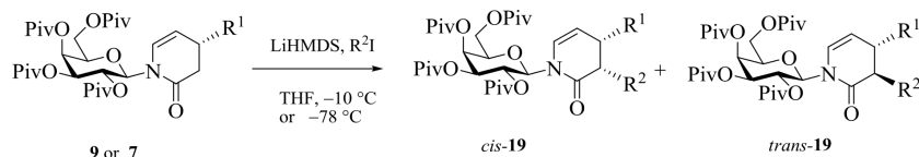
Scheme 8. 3,4-Dialkyl-piperidin-ones.
