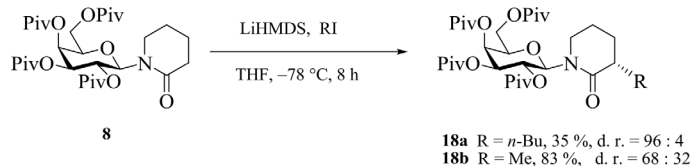
Scheme 7. Alkylation in 3-position; d. r. = ratio of diastereomers.
