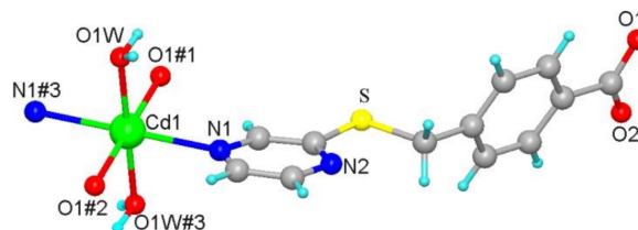
Fig. 1. The connectivity pattern in complex 1 .
