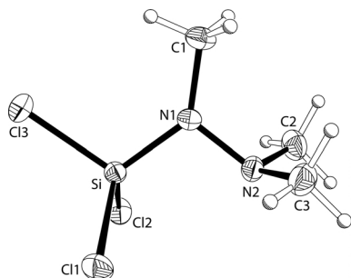
Fig. 5. Molecular structure of \text{Cl}_3\text{SiN}(\text{Me})\text{NMe}_2 ( 2 ) as determined by low-temperature X-ray crystallography (displacement ellipsoids drawn at the 50 % probability level). Selected bond lengths (Å) and angles (deg): Si–N1 1.653(1), Si–Cl1 2.028(1), Si–Cl2 2.026(1), Si–Cl3 2.029(1), N1–N2 1.429(2), N1–C1 1.453(2), N2–C2 1.463(2), N2–C3 1.457(2); N1–Si–Cl1 113.8(1), N1–Si–Cl2 114.8(1), N1–Si–Cl3 108.5(1), C1–Si–Cl2 105.9(1), Cl1–Si–Cl3 107.0(1), N2–N1–Si 105.0(1), C1–N1–Si 134.3(1), C1–N1–N2 120.7(1), N1–N2–C2 111.4(1).
