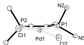
Fig. 5. Reduced structure of 15 showing only the atoms in the chelate ring and directly attached substituents (displacement ellipsoids at the 50 % probability level). The view axis is parallel to the least-squares plane defined by the PCCP fragment of the chelate ring.
