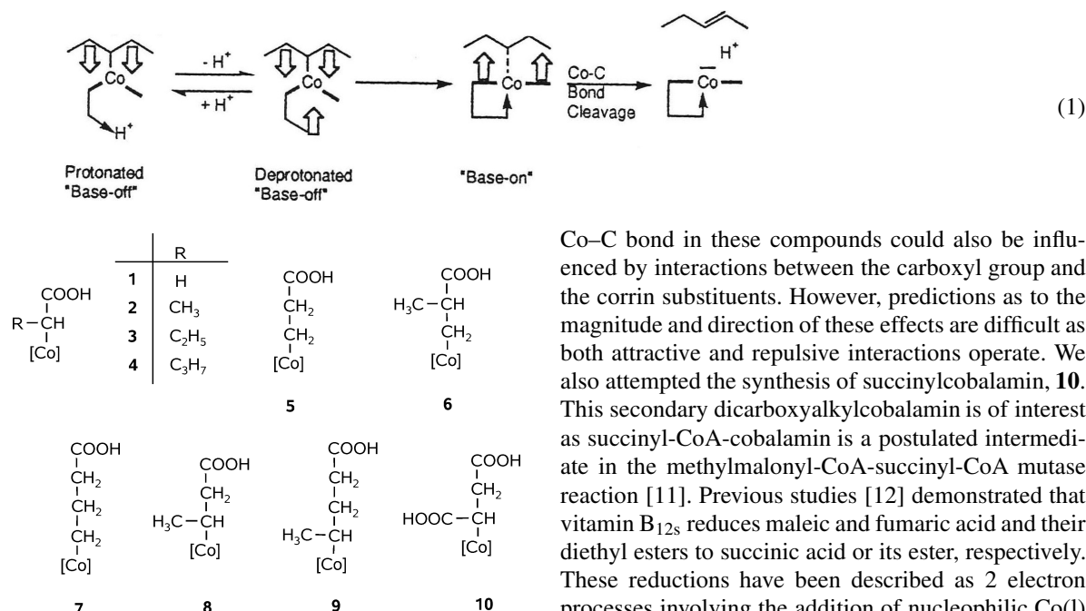
Scheme 1. Carboxyalkylcobalamins studied.
