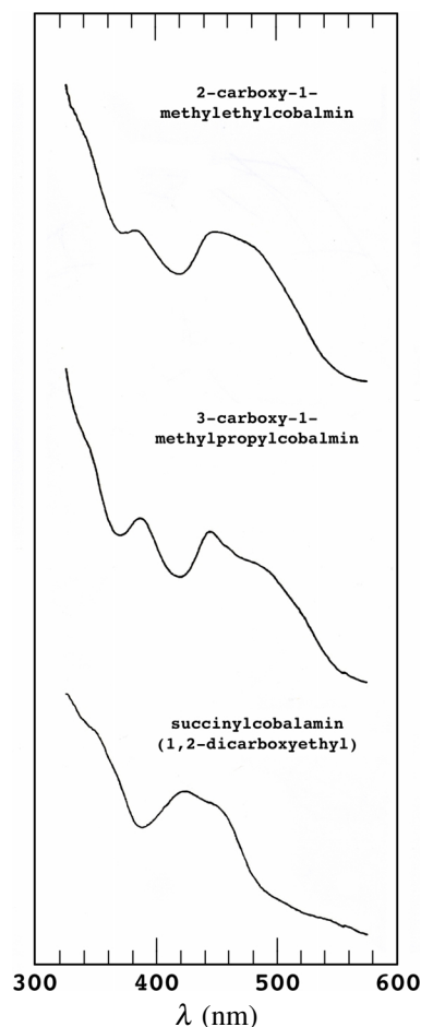
Fig. 2. Absorption spectra of 2-carboxy-1-methylethylcobalamin, 8 , 3-carboxy-1-methylpropylcobalamin, 9 , and of succinylcobalamin, 10 , in glacial acetic acid at 20 °C.
