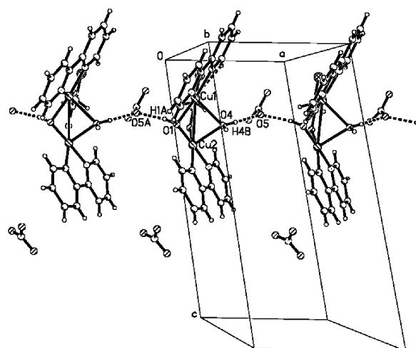
Fig. 3. 1D supramolecular chain along the [100] direction linked by O–H...O hydrogen bonds in the crystal structure of 2 .
