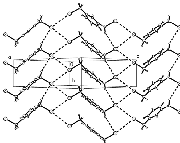
Fig. 7. Packing diagram of compound 2 viewed perpendicular to [101]. Dashed bonds indicate hydrogen bonding or bromine-bromine interactions (see text).
