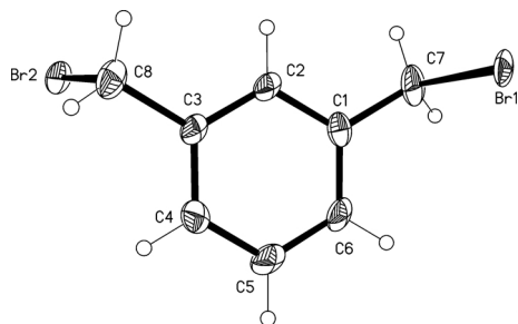
Fig. 2. The molecule of compound 2 in the crystal. Ellipsoids at the 50 % probability level.
