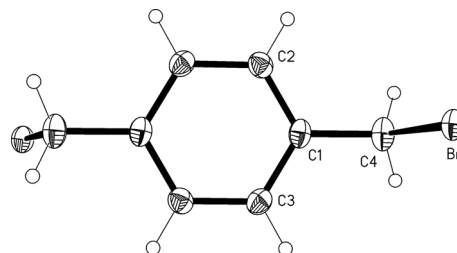
Fig. 1. The molecule of compound 1 in the crystal. Ellipsoids at the 50 % probability level.
