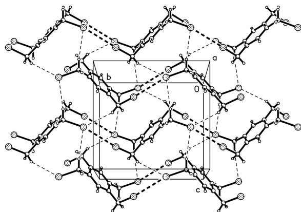
Fig. 10. Packing diagram of compound 4 viewed perpendicular to the yz plane in the region x \approx 0 . Thin dashed lines indicate C-H \cdots Br and thick dashed lines Br \cdots Br interactions. For clarity, the interactions H5B \cdots Br1 and H5A \cdots Br2 are omitted (see text and Table 2).
