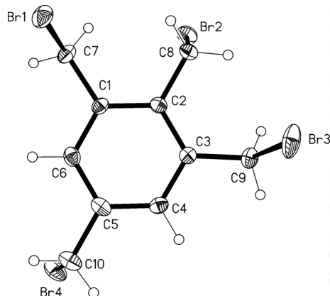
Fig. 5. The molecule of compound 5 in the crystal. Ellipsoids at the 50 % probability level.
