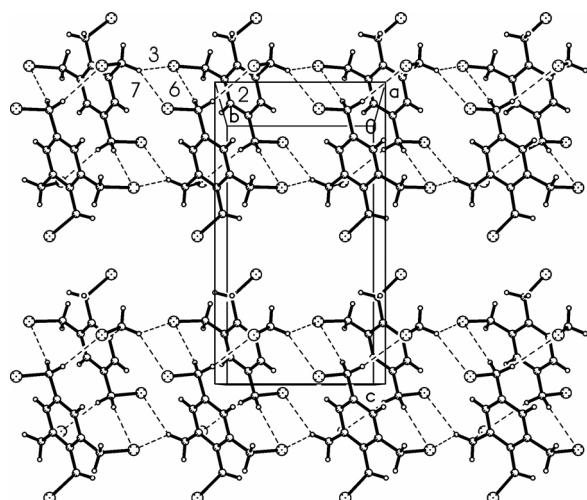
Fig. 11. Packing diagram of compound 5 viewed perpendicular to the yz plane in the region x \approx 0 . Thin dashed lines indicate C-H \cdots Br interactions. H bonds are numbered according to Table 2.
