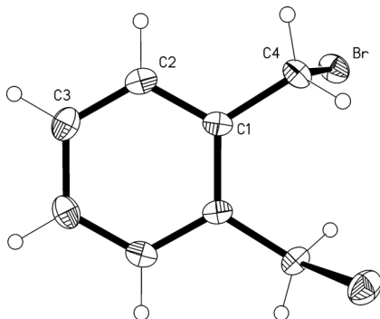
Fig. 3. The molecule of compound 3 in the crystal. Ellipsoids at the 50 % probability level. Intramolecular H bonds are omitted.
