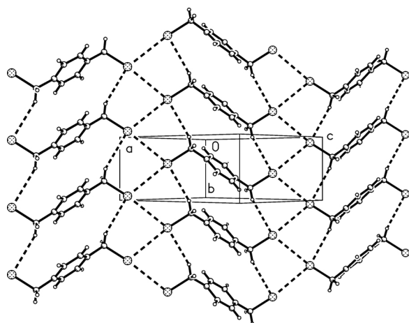
Fig. 6. Packing diagram of compound 1 viewed perpendicular to [101]. Dashed bonds indicate hydrogen bonding or bromine-bromine interactions (see text).
