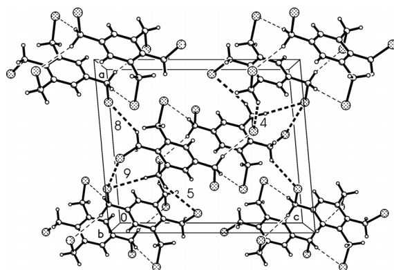
Fig. 12. Packing diagram of compound 5 viewed parallel to the y axis. Thin dashed lines indicate C-H \cdots Br interactions already presented in Fig. 11 (see text); thick dashed lines indicate C-H \cdots Br interactions (numbered according to Table 2) and the short Br \cdots Br contact from the central dimeric unit to the peripheral molecules.
