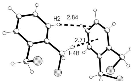
Fig. 8. C–H... \pi interaction in compound 3 (see text). Distances are in Å.
