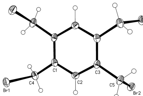
Fig. 4. The molecule of compound 4 in the crystal. Ellipsoids at the 50 % probability level.
