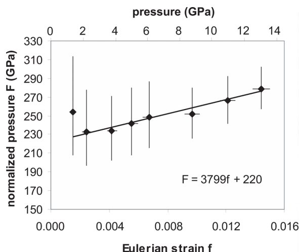
Fig. 7. F - f plot of experimental data on \text{Zr}_{0.1}\text{Ti}_{0.9}\text{O}_2 nano anatase based on the Birch-Murnaghan equation of state. The data are described by a third-order truncation of the equation of state and the linear fit has a slope of 3 K_0 (K' - 4)/2 .
