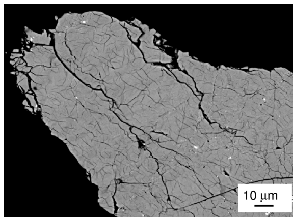
Fig. 7. Scanning electron micrograph of \text{BaSi}_6 showing a number of micro-cracks.
