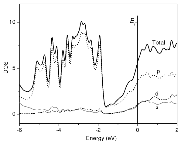
Fig. 5. Density of states (DOS) of \text{BaSi}_6 ; total DOS (solid line), and partial DOS for s (gray line), p (dotted line), and d (dashed line) orbitals.
