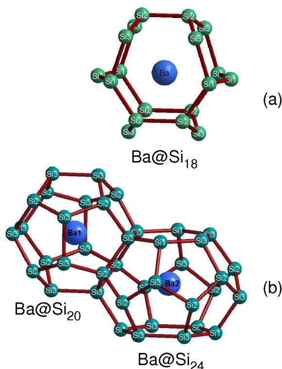
Fig. 4. Comparison of the polyhedra found in the clathrate structures, (a) \text{Ba@Si}_{18} in \text{BaSi}_6 and (b) \text{Ba(1)@Si}_{20} and \text{Ba(2)@Si}_{24} in \text{Ba}_8\text{Si}_{46} . The average Ba-Si distances ( d ) are d_{\text{Ba-Si}} = 3.435 , d_{\text{Ba1-Si}} = 3.365 , and d_{\text{Ba2-Si}} = 3.712 Å.
