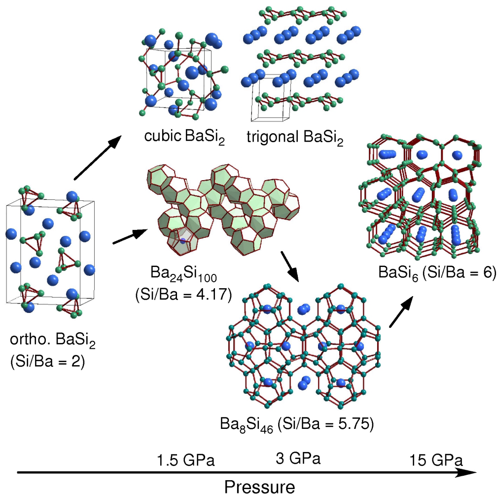
Fig. 1. Schematic illustration of various crystal structures in the binary system Ba-Si found by high-pressure and high-temperature treatments; orthorhombic \text{BaSi}_2 is transformed to trigonal \text{BaSi}_2 and cubic \text{BaSi}_2 .
