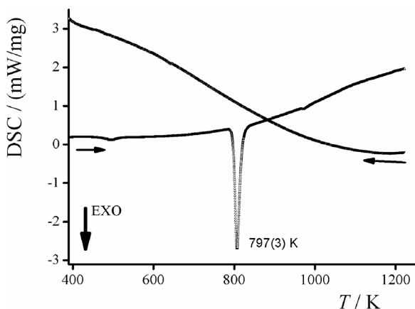
Fig. 2. Differential scanning calorimetry measurement of SrSi 6 at ambient pressure. With increasing temperature, the decomposition of the metastable high-pressure phase SrSi 6 into the products SrSi 2 and Si which are thermodynamically stable at ambient pressure is detected by an exothermic peak at 797(3) K (onset temperature).
