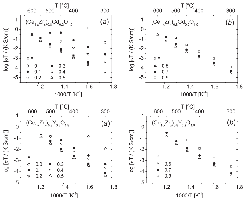
Fig. 4. Temperature dependence of the bulk conductivities of the (\text{Ce}_{1-x}\text{Zr}_x)_{0.8}\text{Gd}_{0.2}\text{O}_{1.9} solid solutions: a) x = 0.0–0.5 ; b) x = 0.5–0.9 .
